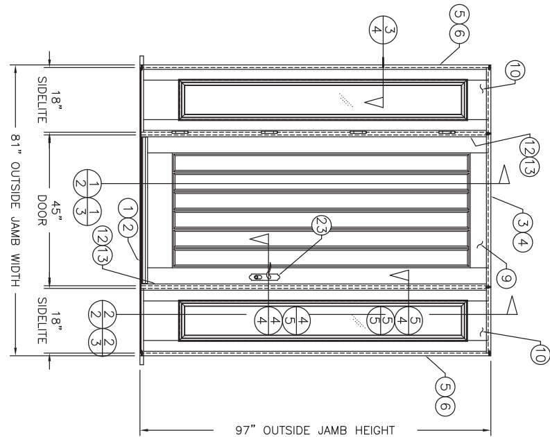
SINGLE UNIT W/ 2 SIDELITES (OXO) SCALE: 1/2" = 1'-0"
